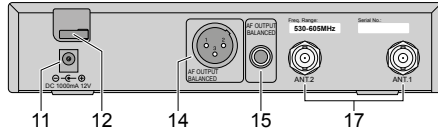
Fig.3 Connections
